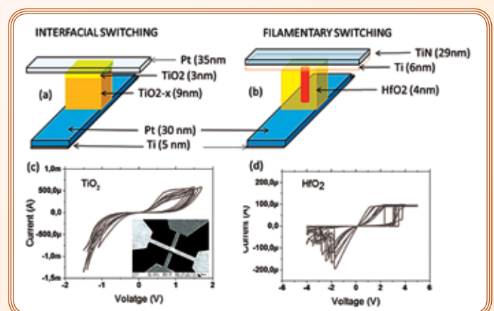
Figure 1: Schematic of our fabricated nanoscale OxRAM devices for (a) \text{TiO}_2 and (b) \text{HfO}_2 stacks. (c) and (d) show corresponding IV curves with an Inset SEM image of the \text{TiO}_2 device [2].
